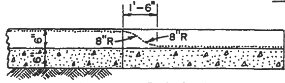
SECTION ELEVATION AT GUTTER LINE
